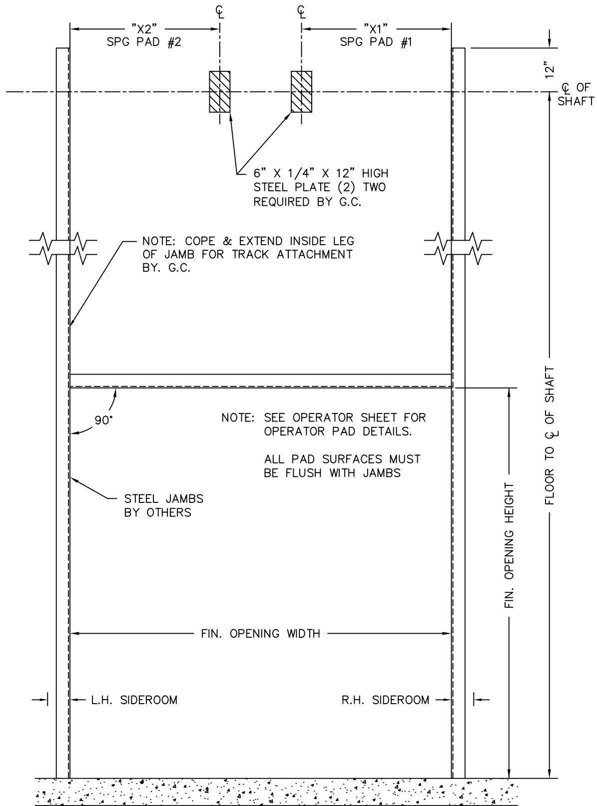
INTERIOR ELEVATION
