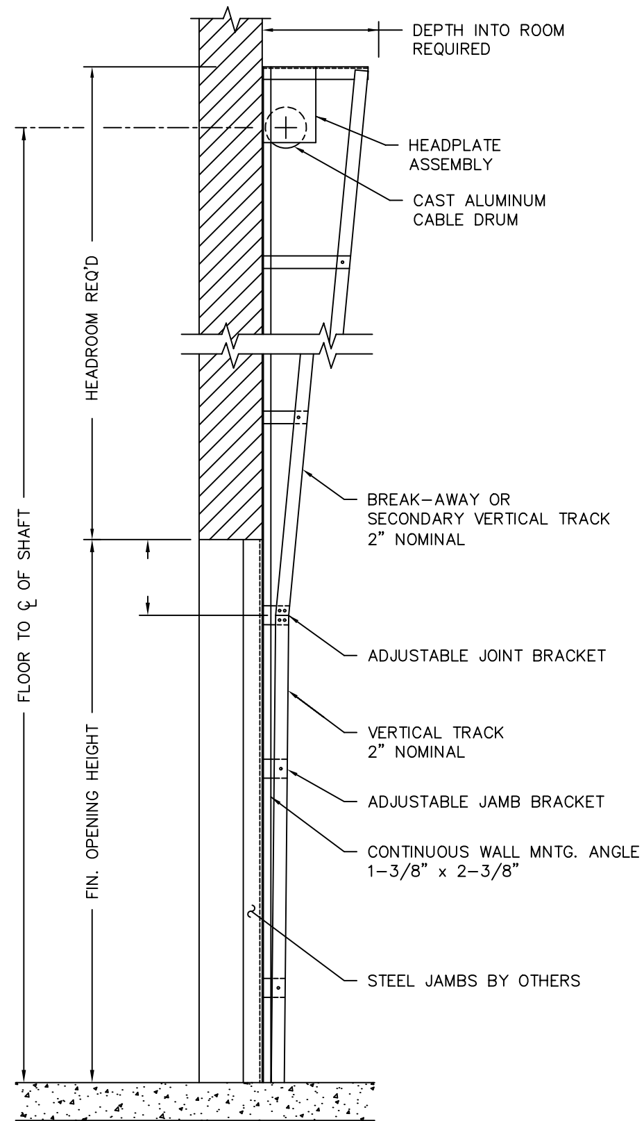
SIDE VIEW OF MOUNTED TRACK
