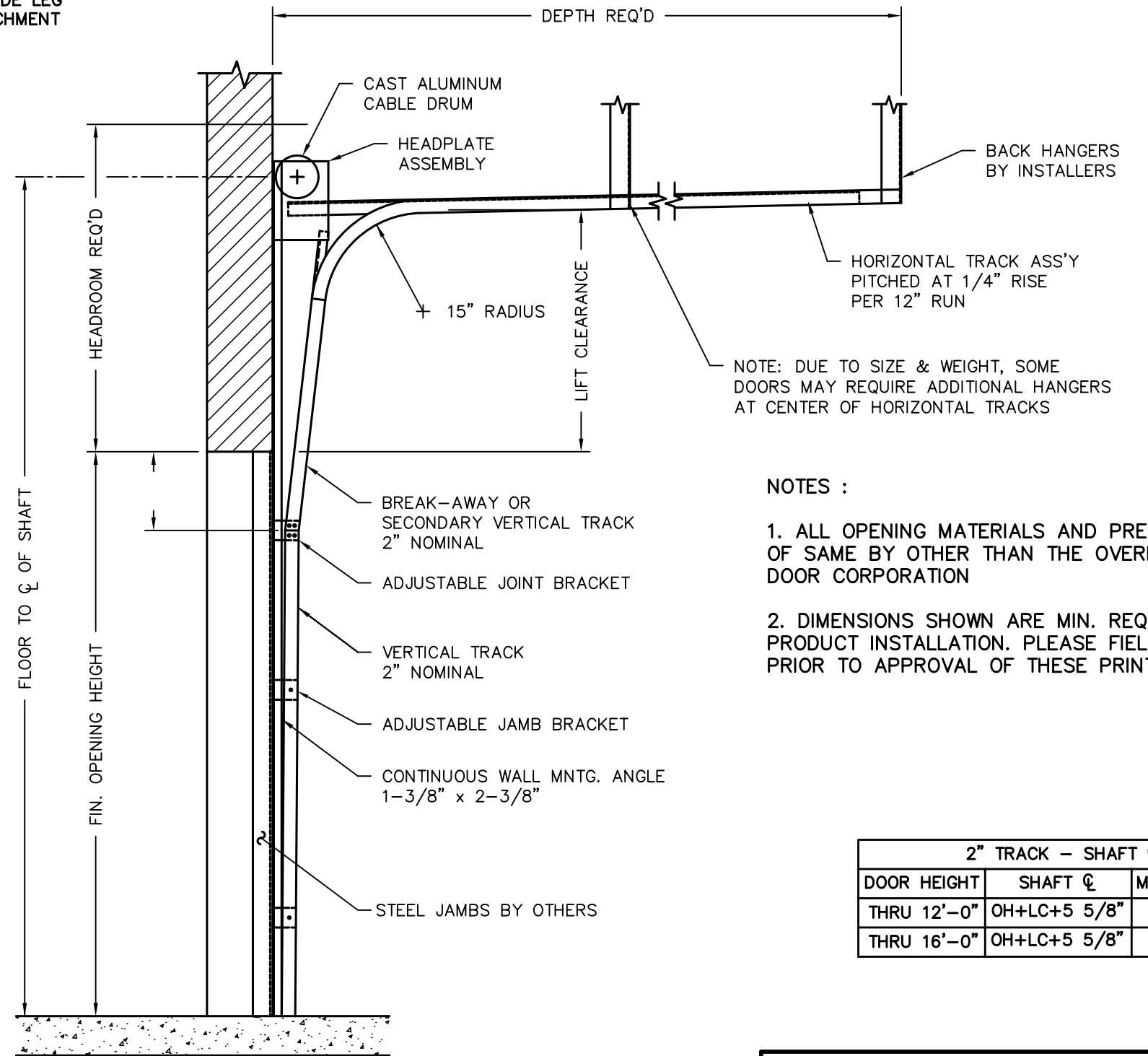
SIDE VIEW OF MOUNTED TRACK
