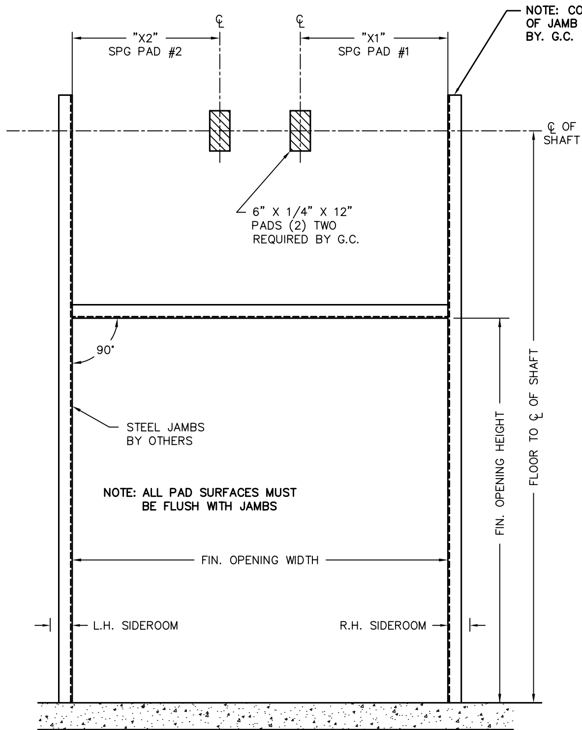
INTERIOR ELEVATION
